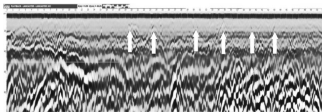
FIG. 7. GPR output image indicating the presence of subsurface anomalies (arrows) possibly indicative of additional graves.
